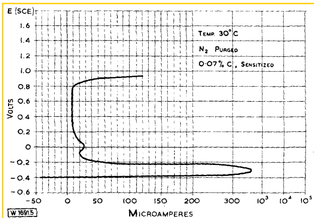
Fig. 5. Polarisation characteristics of 18Cr10Ni in 1 N \text{H}_2\text{SO}_4
