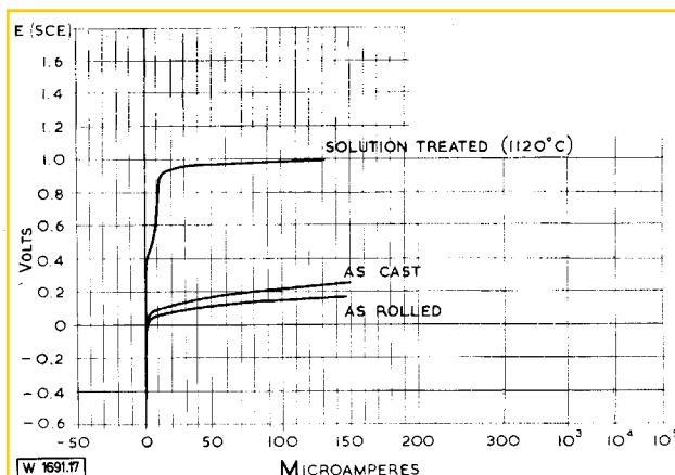
Fig. 17. Effect of solution treatment on polarisation characteristics in 3% NaCl
