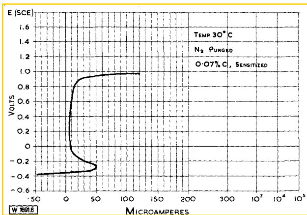
Fig. 6. Polarisation characteristics of 18Cr10Ni3Mo in 1 N \text{H}_2\text{SO}_4
