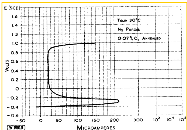
Fig. 8. Polarisation characteristics of 18Cr10Ni3Mo1Nb in 1N H_2SO_4
