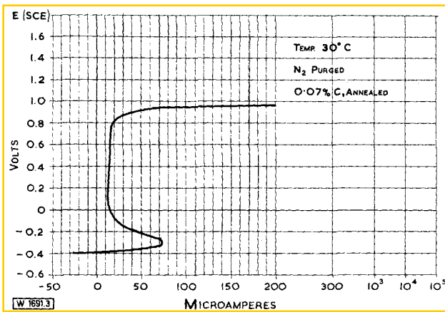
Fig. 3. Polarisation characteristics of 18Cr10Ni3Mo in 1 N \text{H}_2\text{SO}_4
