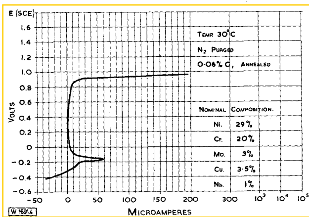
Fig. 4. Polarisation characteristics of L'ANGALLOY 20V special stainless steel in 1 N \text{H}_2\text{SO}_4
