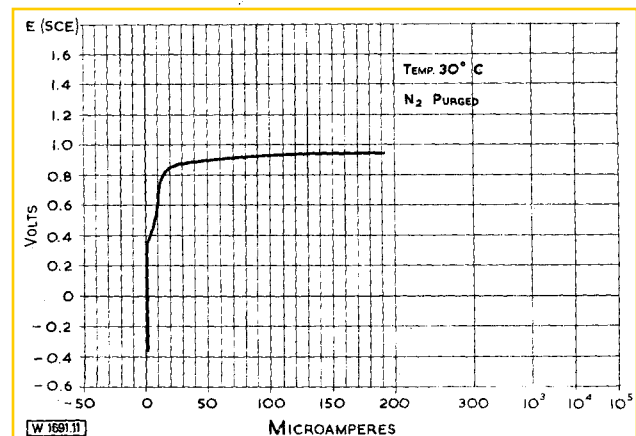
Fig. 11. Polarisation characteristics of Ferralium alloy in 3% NaCl
