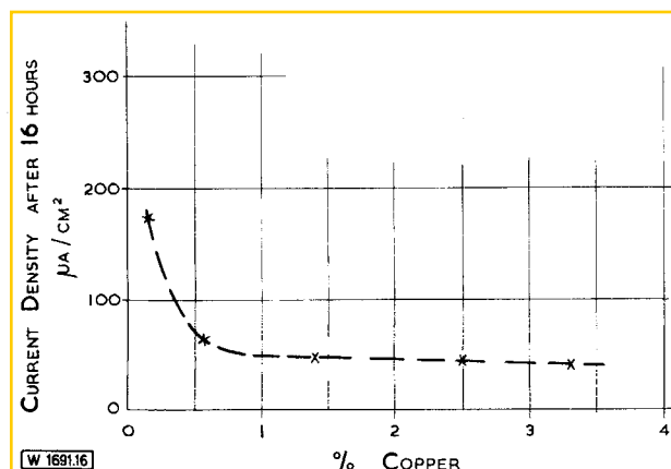
Fig. 16. Effect of copper content on pitting resistance in 3% NaCl
